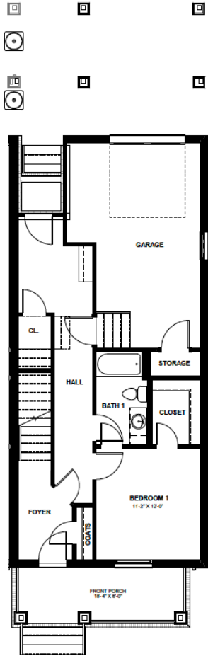
LOT 1 - 1ST FLOOR
