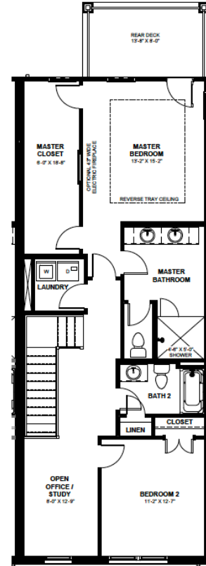
LOT 1 - 3RD FLOOR
