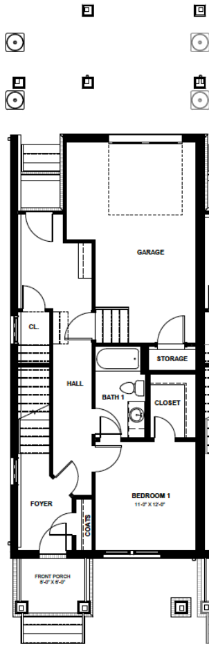
LOT 6 - 1ST FLOOR
